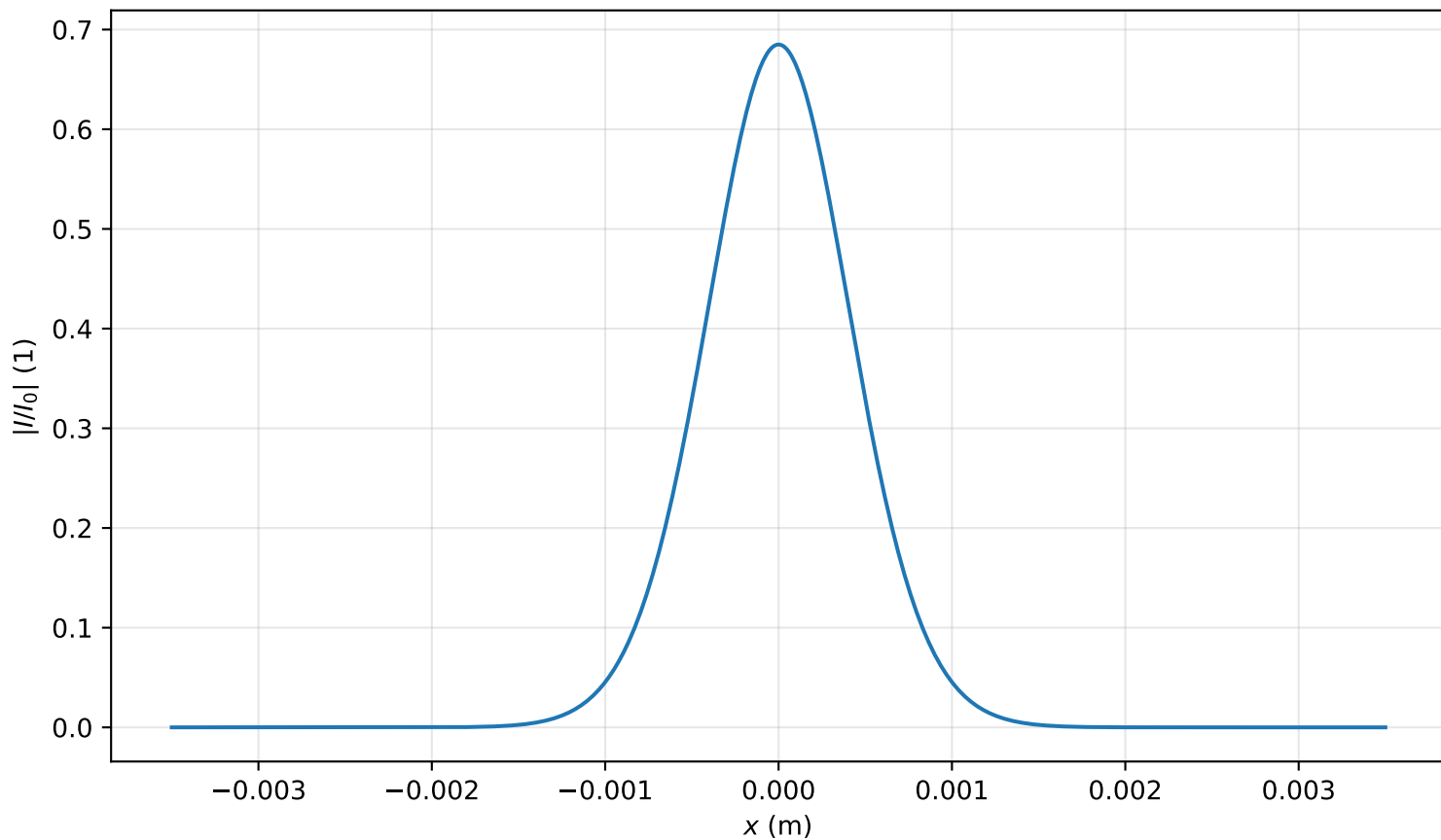
Intensity profile I(x, y = 0, z = 1.672m)/I_0 , P_{in}=0.2P_{cr} , artificial time
